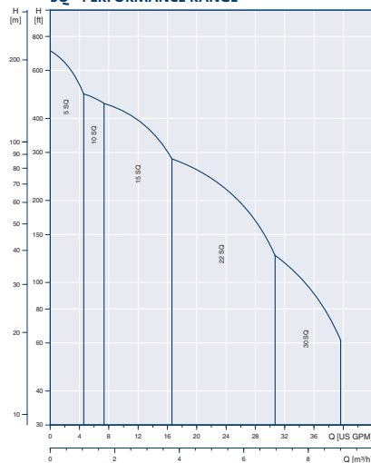
SQ - PERFORMANCE RANGE
