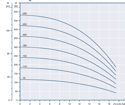
22 SQ ISO 9906 Annex A
