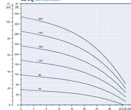
30 SQ ISO 9906 Annex A
