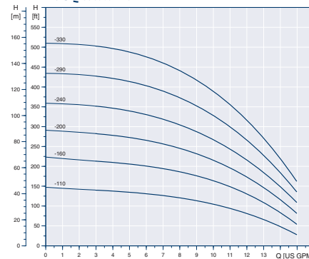
10 SQ ISO 9906 Annex A
